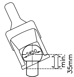
Fig. 1: Towing vehicle ball rod
