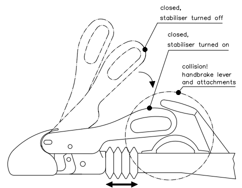
Fig. 5: Switching on stabiliser
