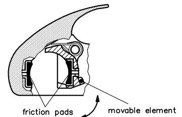
Fig. 9: Location of friction pads
